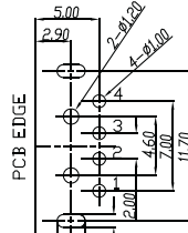
COMPONENT SIDE (PCB LAYOUT)
